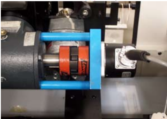
The Servo3000 is supplied with an encoder coupled to the press. The encoder signal represents press speed and press position.
